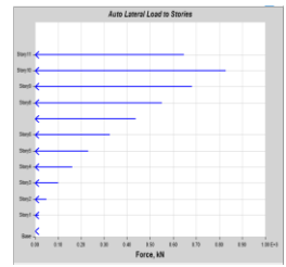
Fig 9.3 lateral Load at Zone 3(X) by Static Analysis
